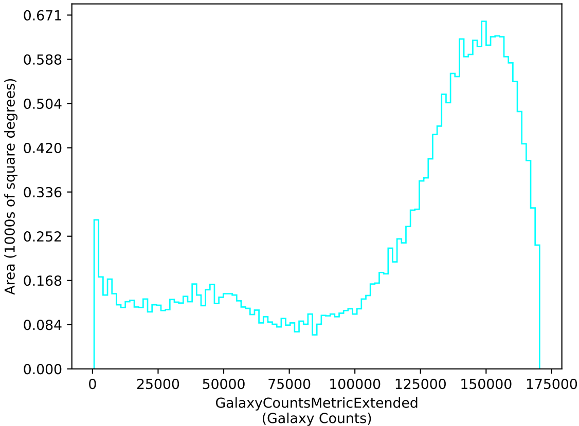
weather_cloudso6v3.5_10yrs u: GalaxyCountsMetricExtended
