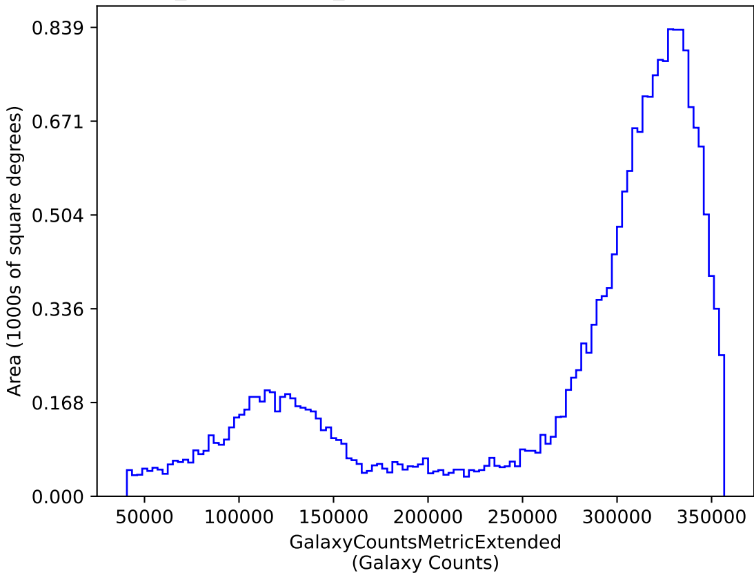
weather_cloudso6v3.5_10yrs y: GalaxyCountsMetricExtended
