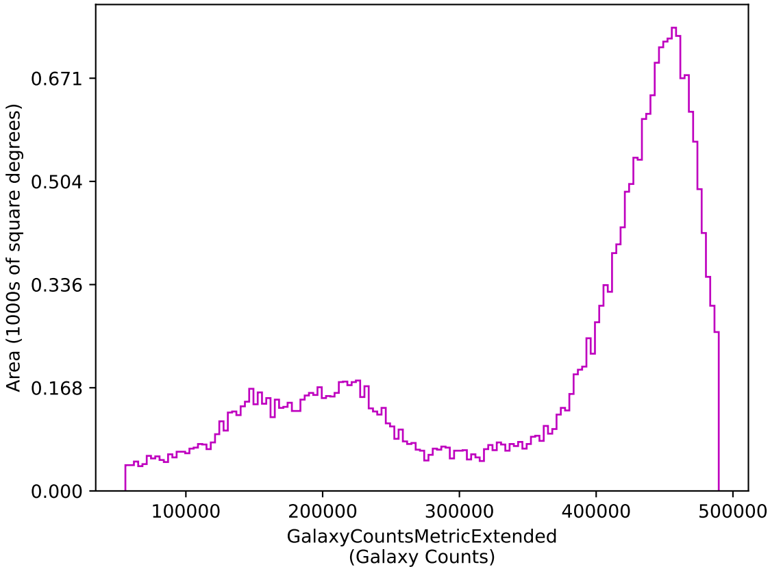
weather_cloudso6v3.5_10yrs z: GalaxyCountsMetricExtended
