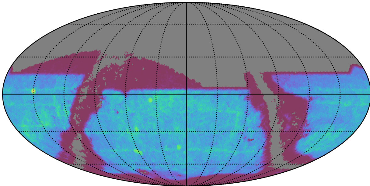
weather_cloudso6v3.5_10yrs : SNSLMetric
