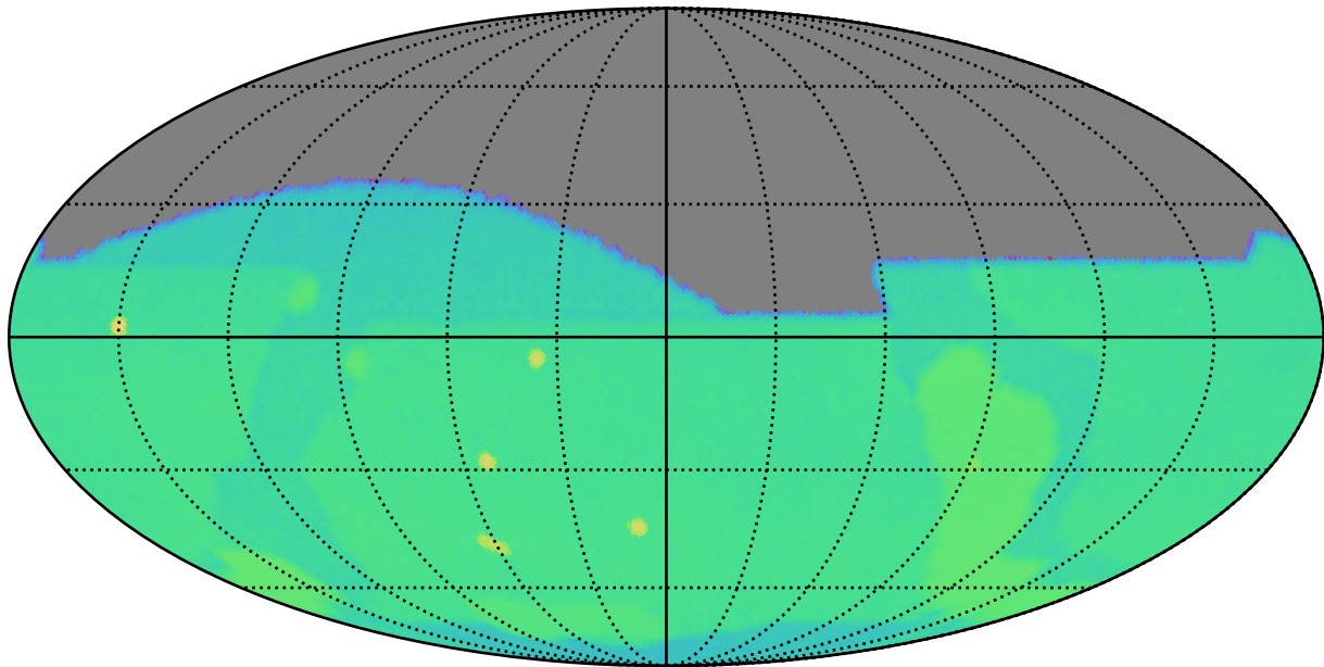
weather_cloudso6v3.5_10yrs g: SurfaceBrightLimit
