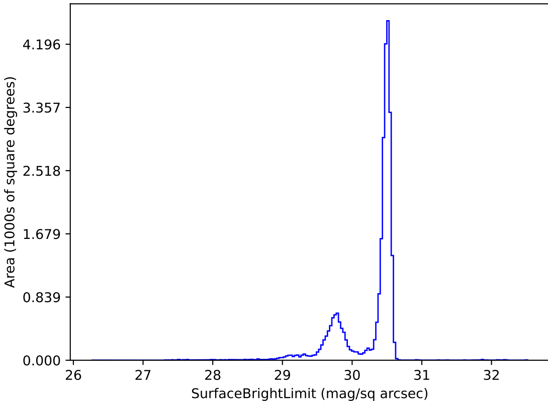
weather_cloudso6v3.5_10yrs r: SurfaceBrightLimit
