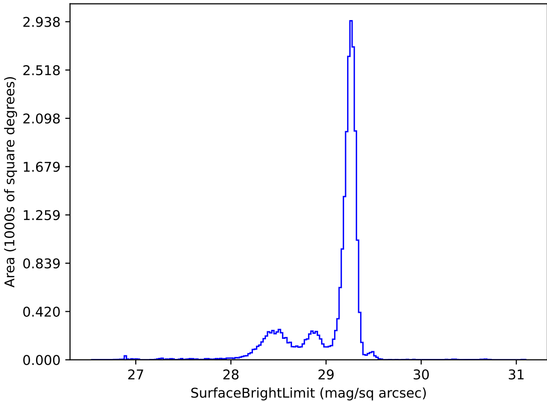
weather_cloudso6v3.5_10yrs u: SurfaceBrightLimit
