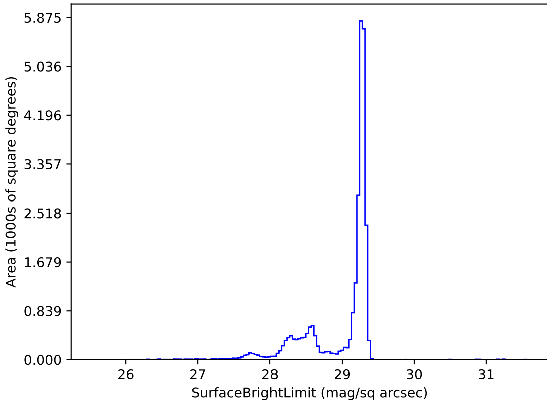
weather_cloudso6v3.5_10yrs z: SurfaceBrightLimit
