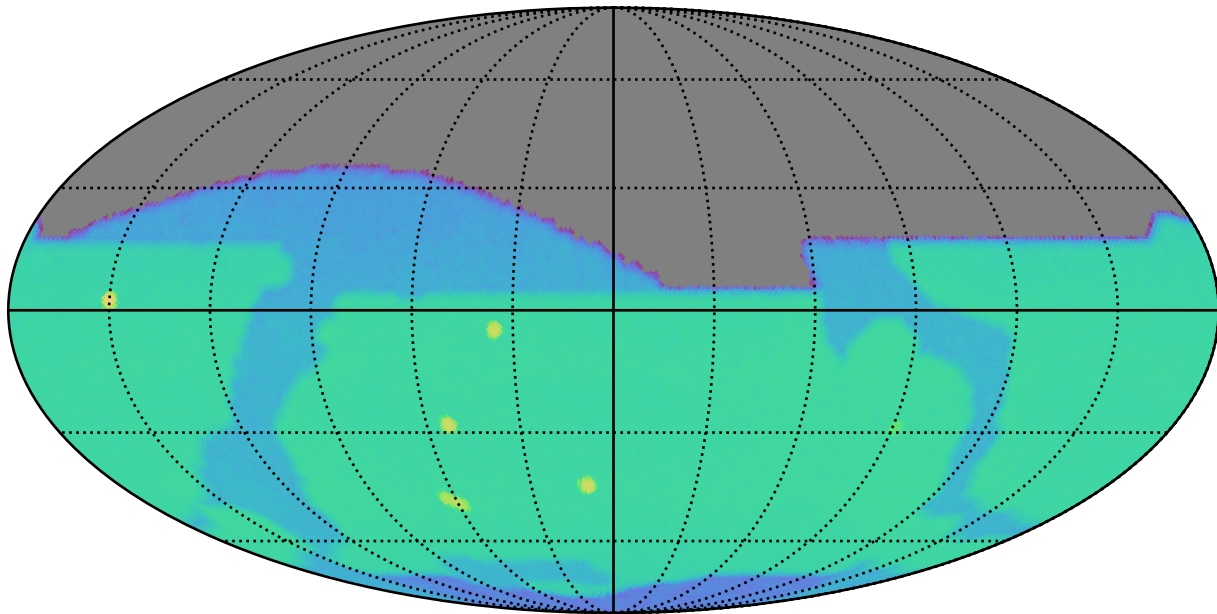
weather_cloudso6v3.5_10yrs z: SurfaceBrightLimit
