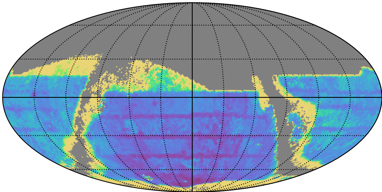
weather_cloudso6v3.5_10yrs : TDC_accuracy
