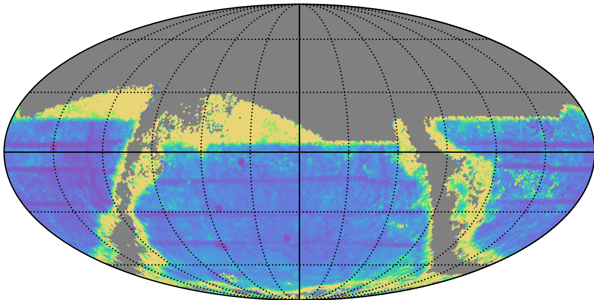
weather_cloudso6v3.5_10yrs : TDC_cadence
