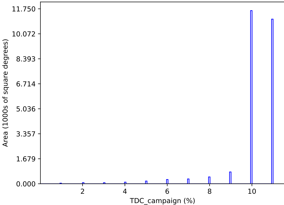
weather_cloudso6v3.5_10yrs : TDC_campaign
