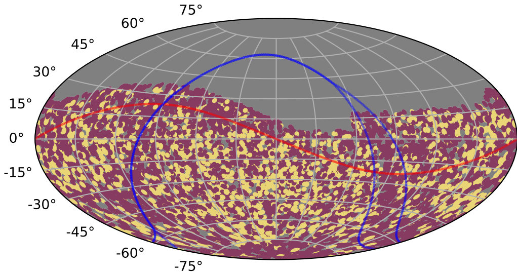
weather_cloudso6v3.5_10yrs : TDEsPopMetric_prepeak
