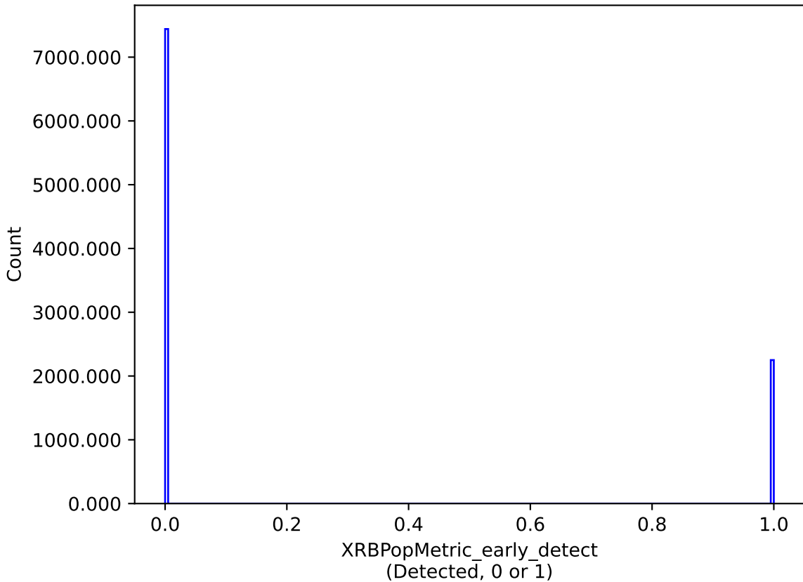
weather_cloudso6v3.5_10yrs : XRBPoMetric_early_detect
