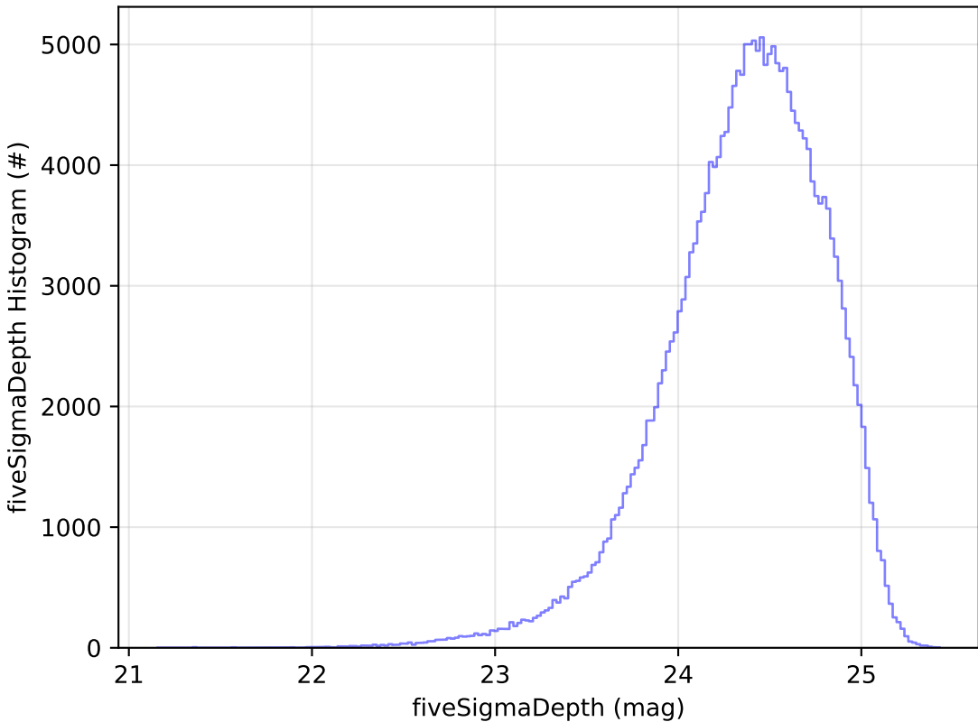
weather_cloudso6v3.5_10yrs g: fiveSigmaDepth Histogram
