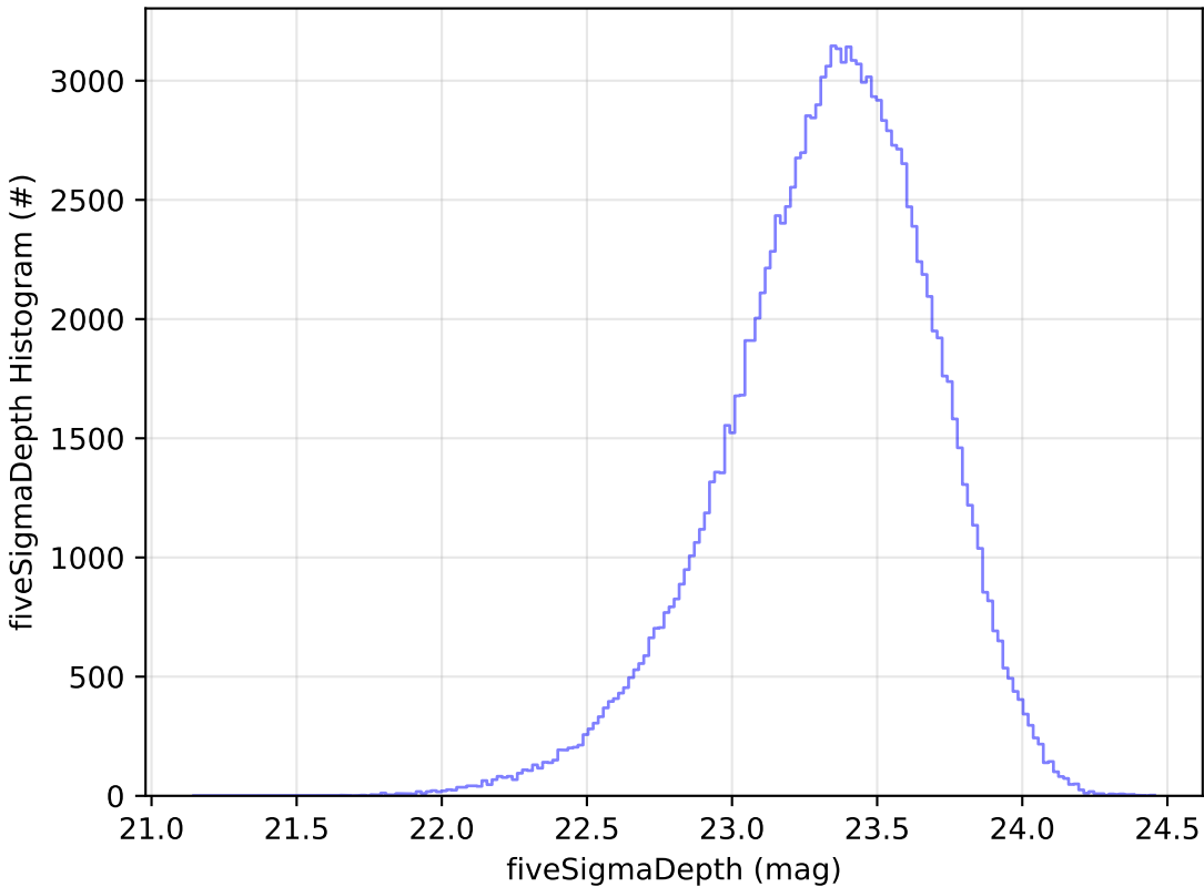
weather_cloudso6v3.5_10yrs u: fiveSigmaDepth Histogram
