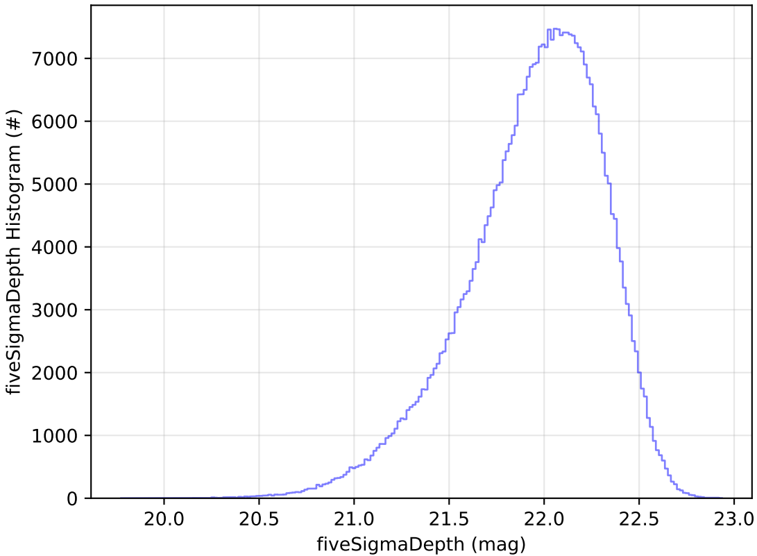
weather_cloudso6v3.5_10yrs y: fiveSigmaDepth Histogram
