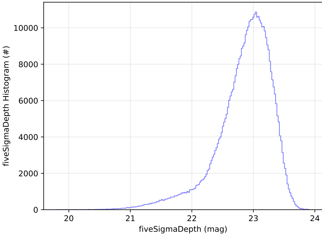
weather_cloudso6v3.5_10yrs z: fiveSigmaDepth Histogram
