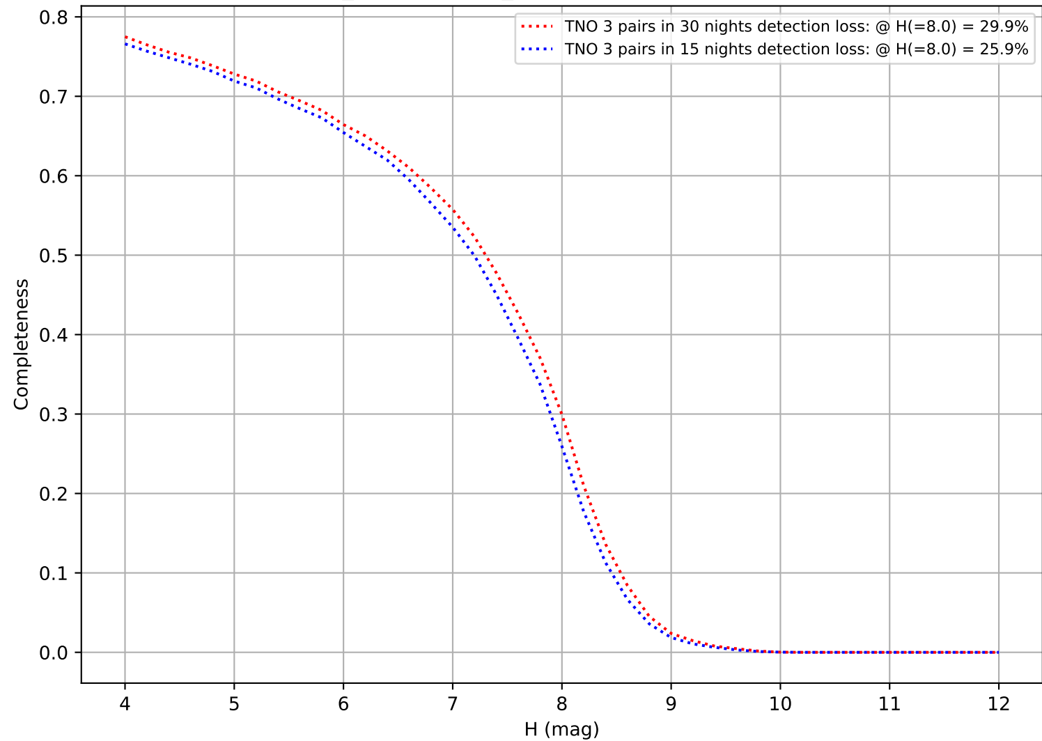
weather_cloudso6v3.5_10yrs: DifferentialCompleteness
