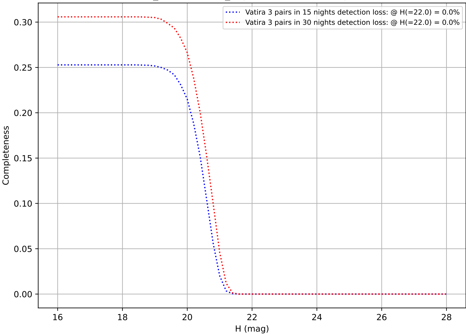
weather_cloudso6v3.5_10yrs: DifferentialCompleteness
