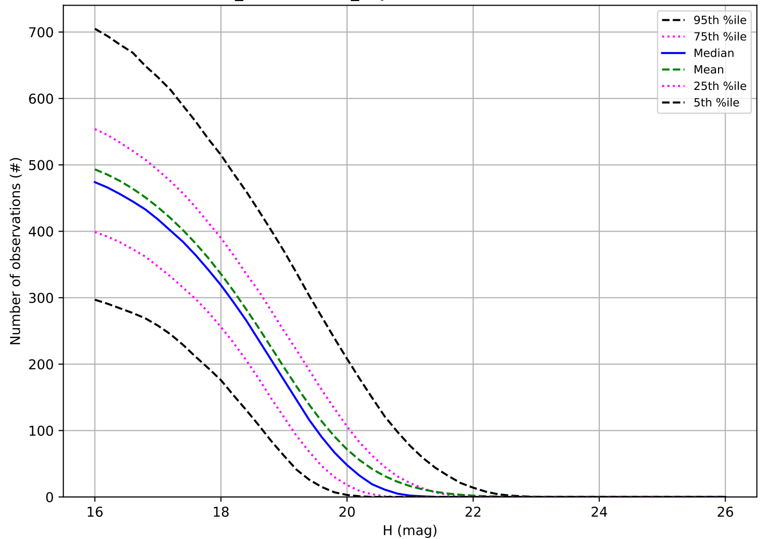
weather_cloudso6v3.5_10yrs: Number of observations MBA
