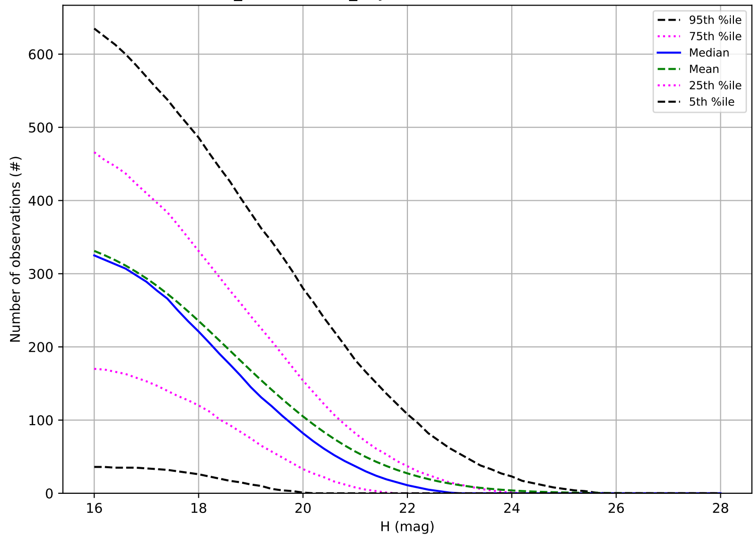
weather_cloudso6v3.5_10yrs: Number of observations NEO
