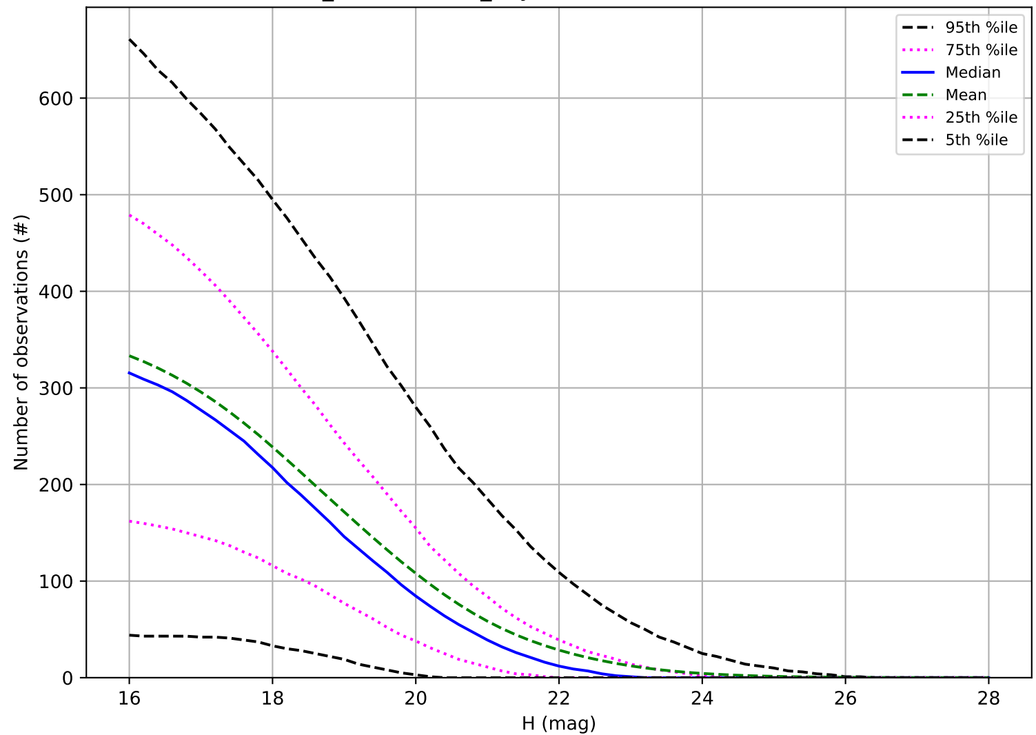
weather_cloudso6v3.5_10yrs: Number of observations PHA
