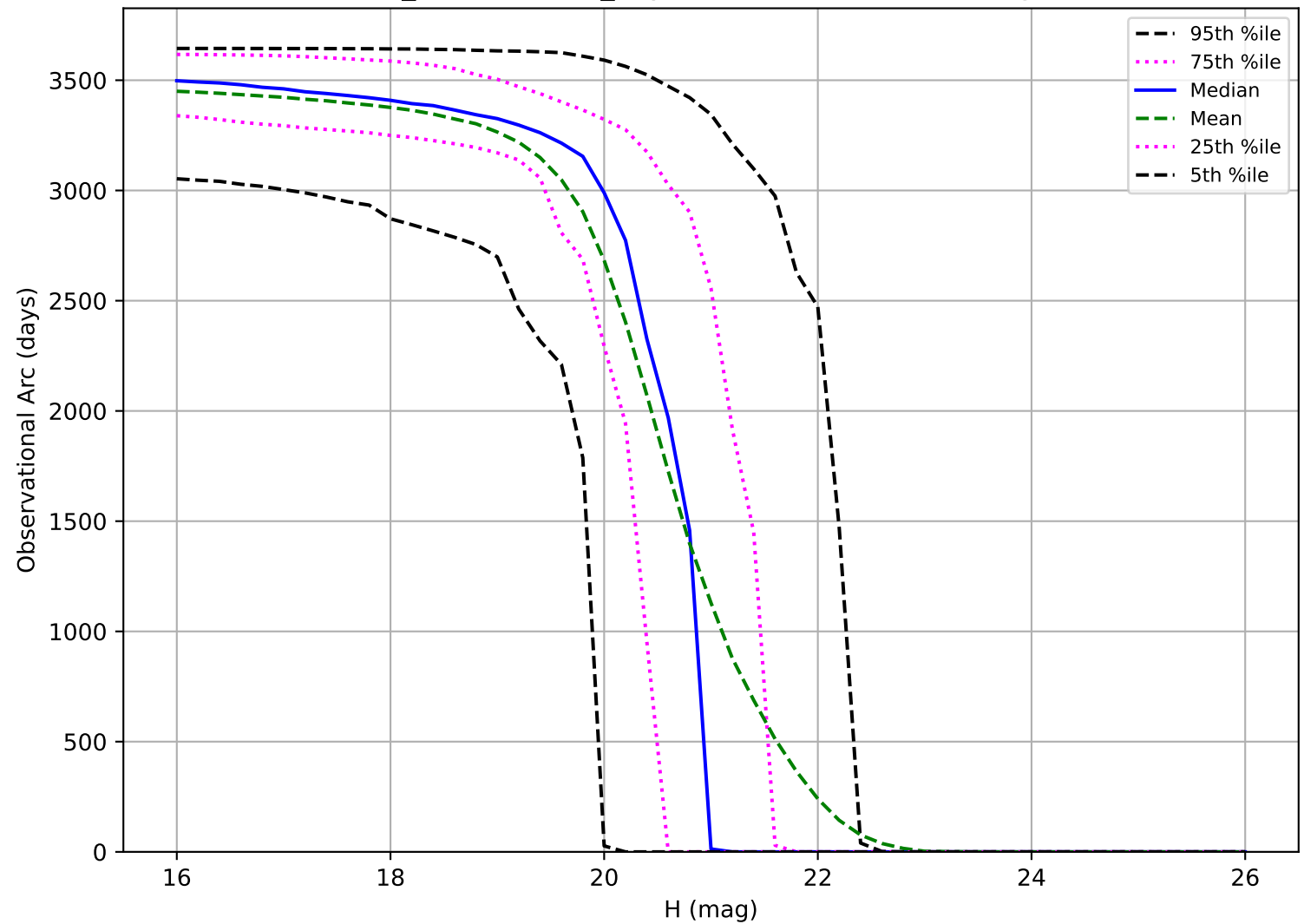
weather_cloudso6v3.5_10yrs: Observational Arc Length MBA
