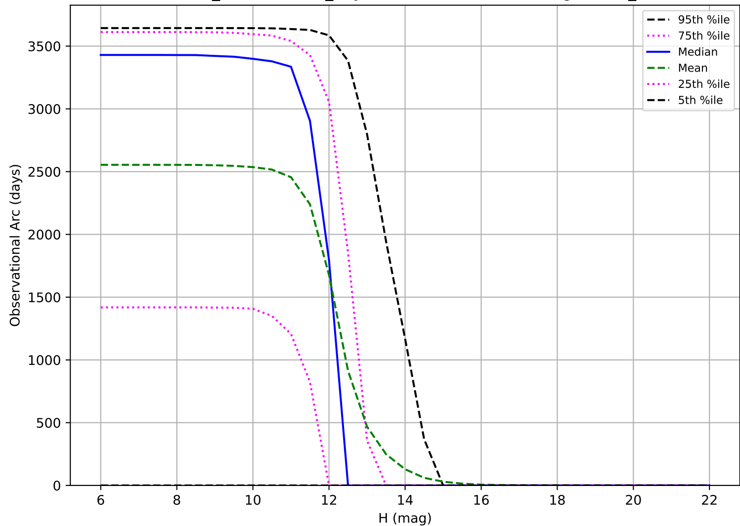
weather_cloudso6v3.5_10yrs: Observational Arc Length OCC_r20
