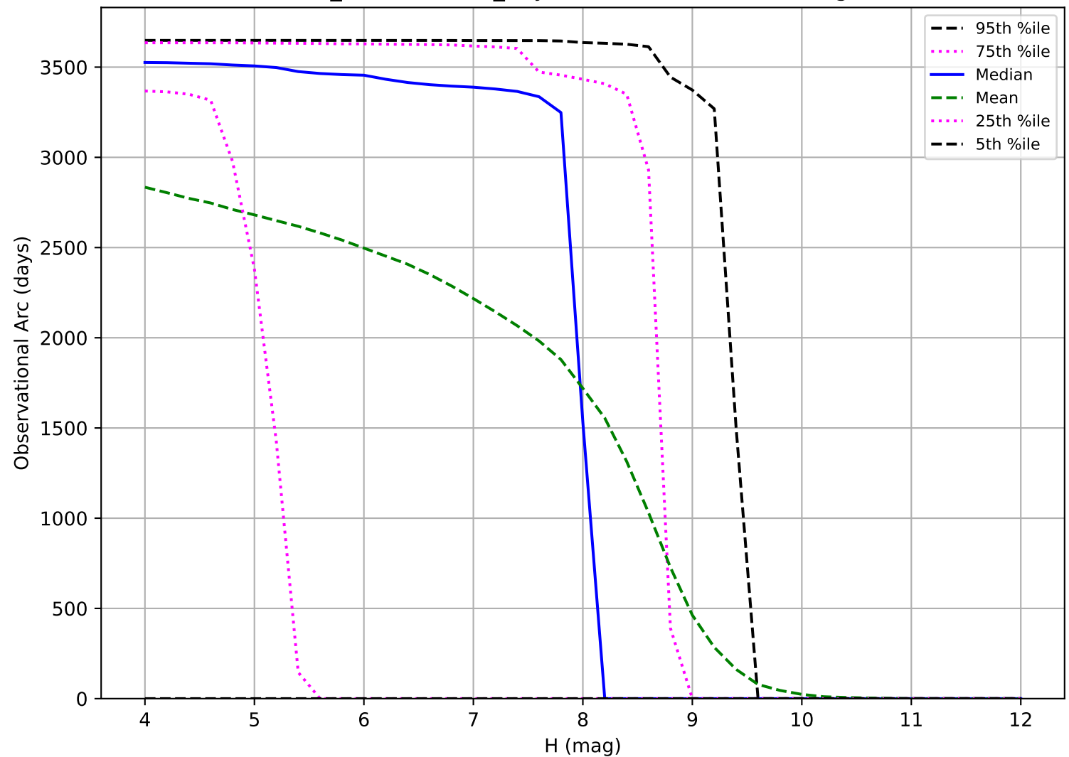
weather_cloudso6v3.5_10yrs: Observational Arc Length TNO
