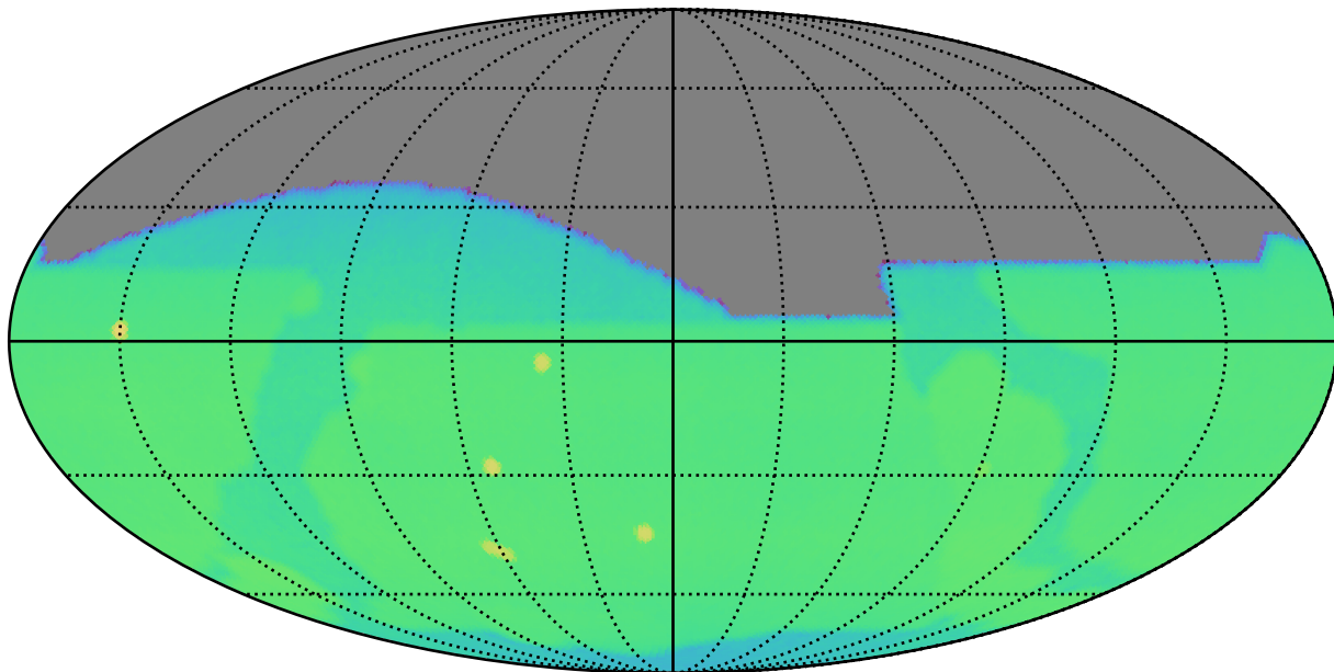
weather_cloudso8v3.5_10yrs : CoaddM5
