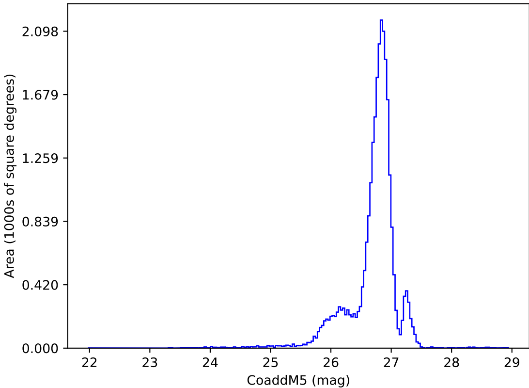
weather_cloudso8v3.5_10yrs g: CoaddM5
