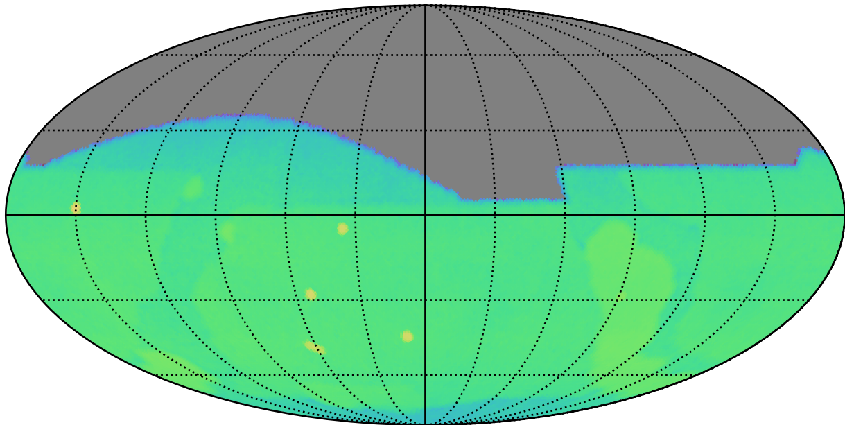
weather_cloudso8v3.5_10yrs g: CoaddM5
