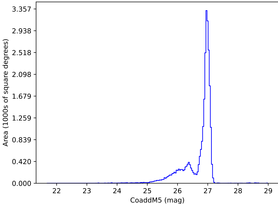
weather_cloudso8v3.5_10yrs r: CoaddM5
