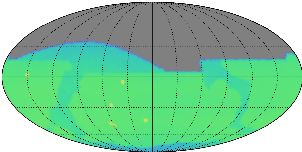
weather_cloudso8v3.5_10yrs r: CoaddM5
