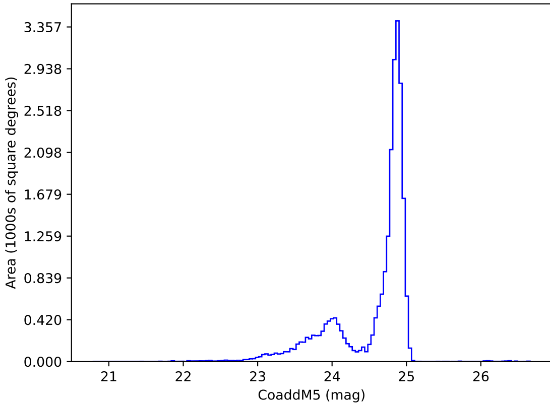
weather_cloudso8v3.5_10yrs y: CoaddM5
