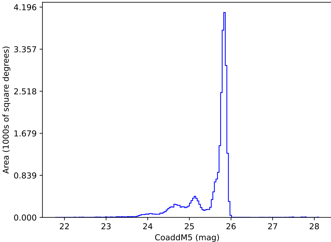
weather_cloudso8v3.5_10yrs z: CoaddM5
