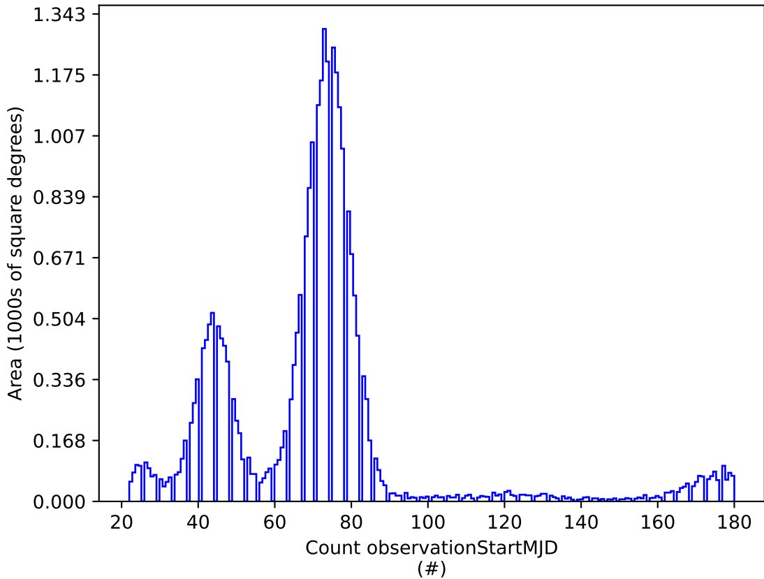
weather_cloudso8v3.5_10yrs g: Count observationStartMJD
