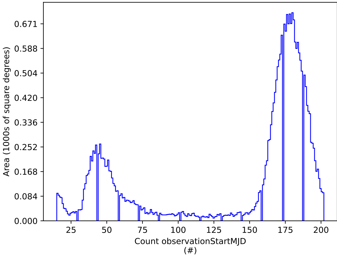
weather_cloudso8v3.5_10yrs z: Count observationStartMJD
