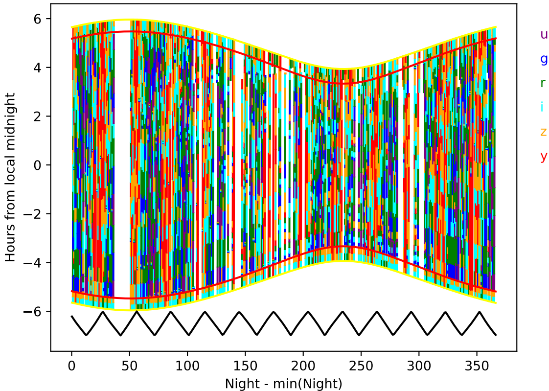
weather_cloudso8v3.5_10yrs year 4-5: Hourglass
