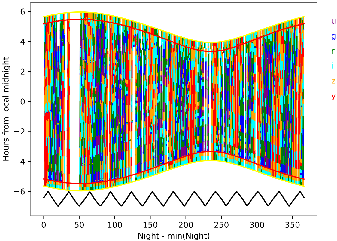
weather_cloudso8v3.5_10yrs year 6-7: Hourglass
