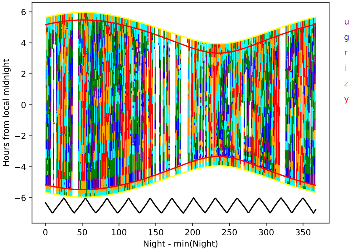
weather_cloudso8v3.5_10yrs year 7-8: Hourglass
