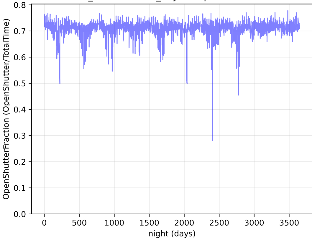
weather_cloudso8v3.5_10yrs : OpenShutterFraction
