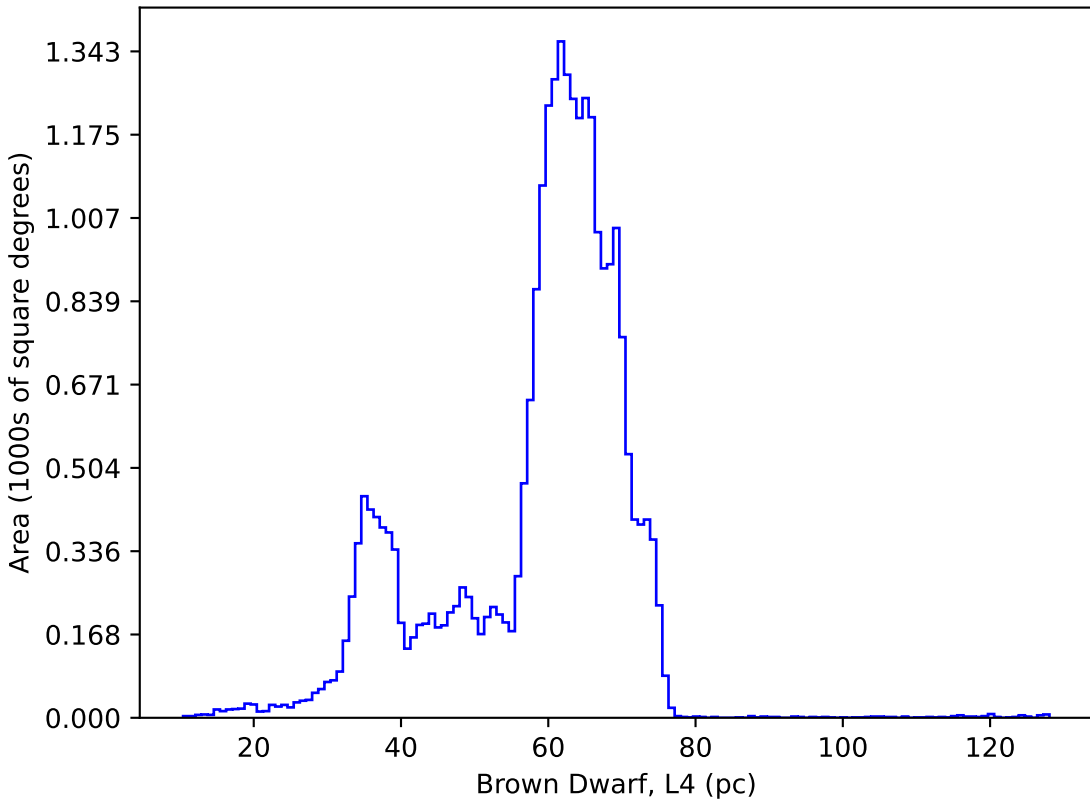
weather_cloudso8v3.5_10yrs : Brown Dwarf, L4
