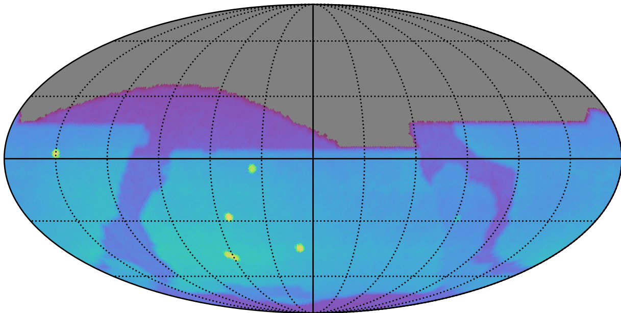
weather_cloudso8v3.5_10yrs : Brown Dwarf, L4
