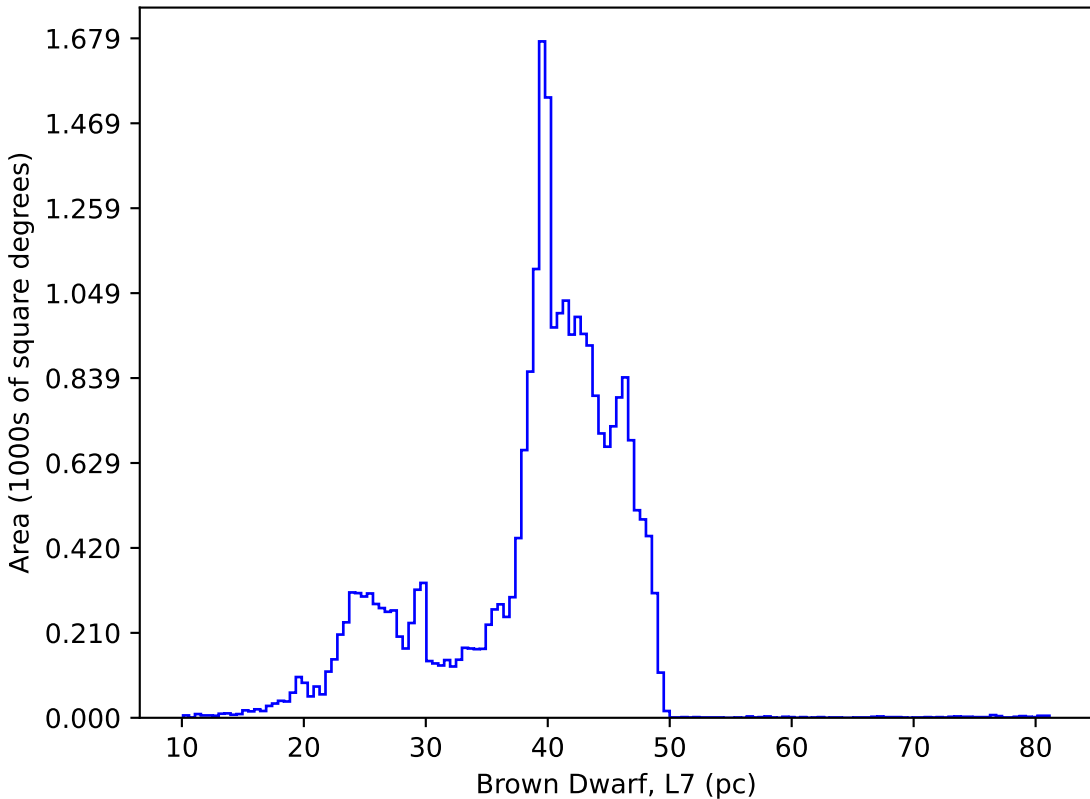
weather_cloudso8v3.5_10yrs : Brown Dwarf, L7
