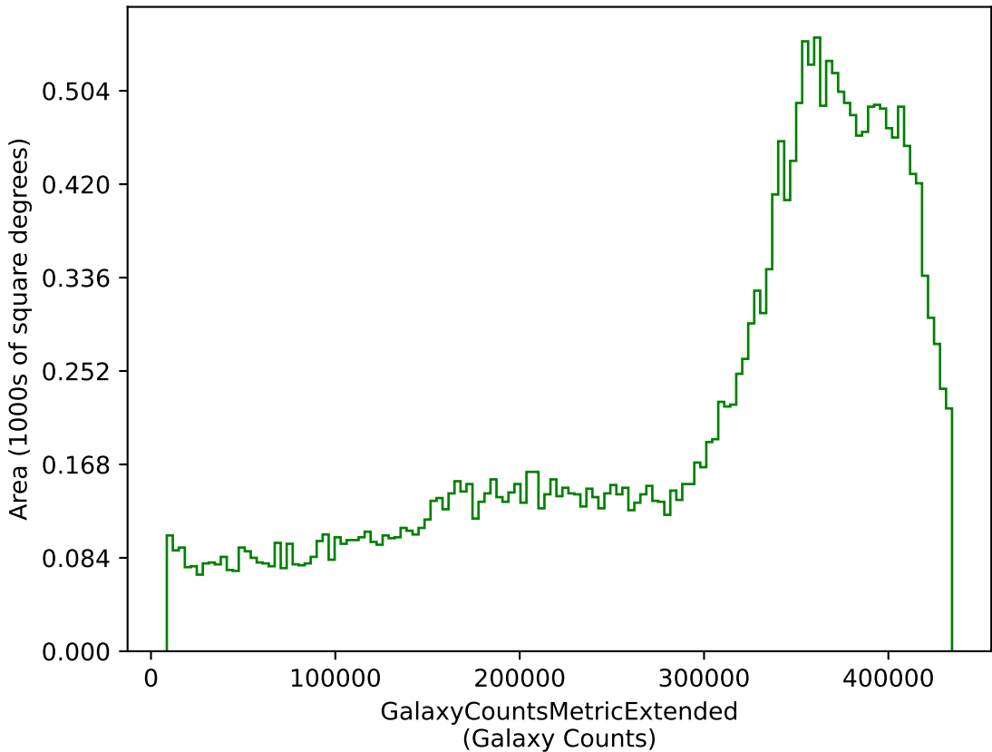
weather_cloudso8v3.5_10yrs g: GalaxyCountsMetricExtended
