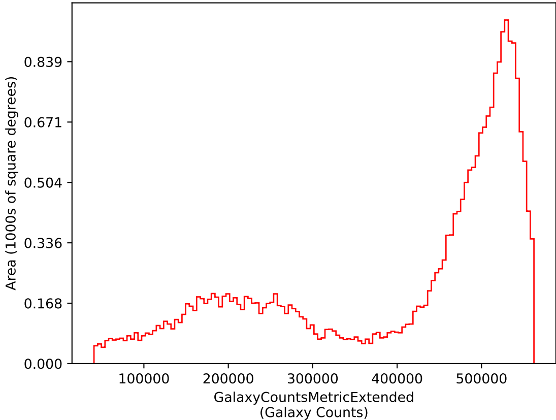
weather_cloudso8v3.5_10yrs i: GalaxyCountsMetricExtended
