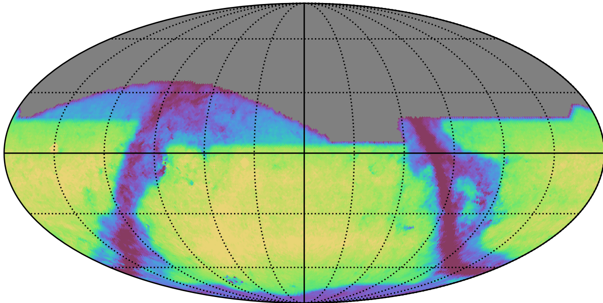
weather_cloudso8v3.5_10yrs i: GalaxyCountsMetricExtended
