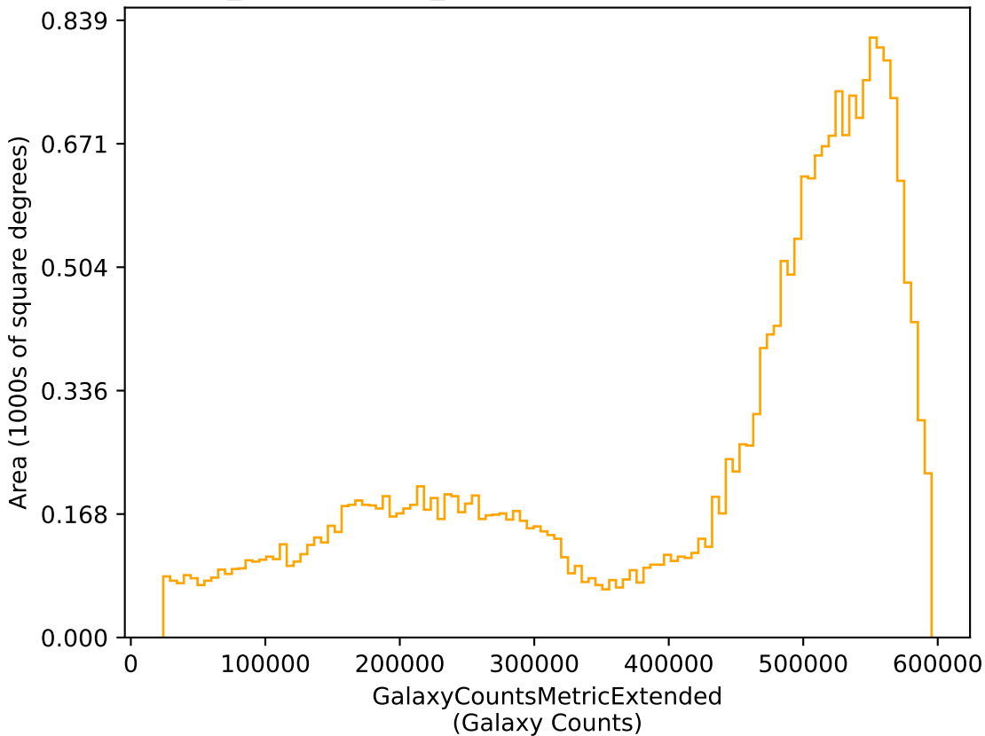
weather_cloudso8v3.5_10yrs r: GalaxyCountsMetricExtended
