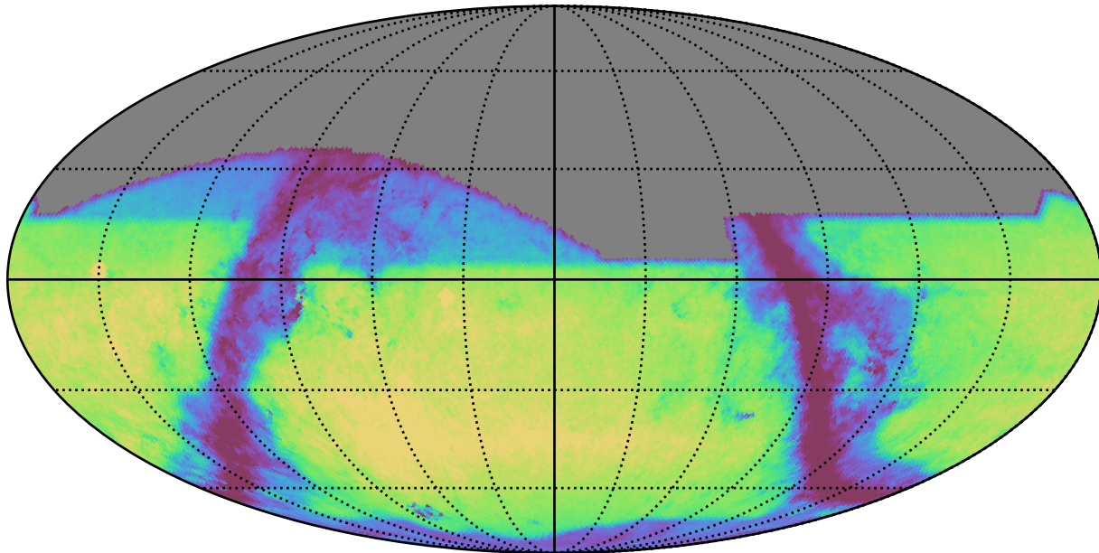
weather_cloudso8v3.5_10yrs r: GalaxyCountsMetricExtended
