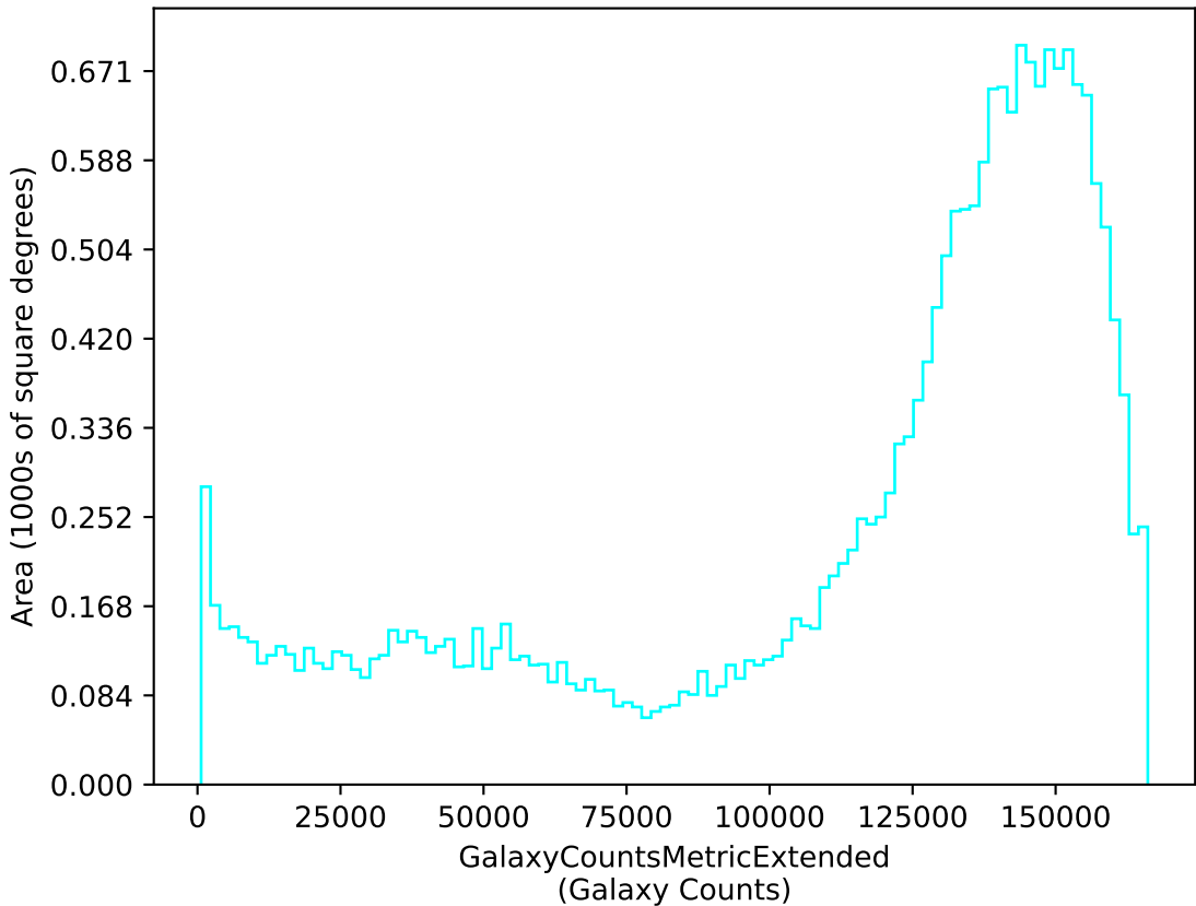
weather_cloudso8v3.5_10yrs u: GalaxyCountsMetricExtended
