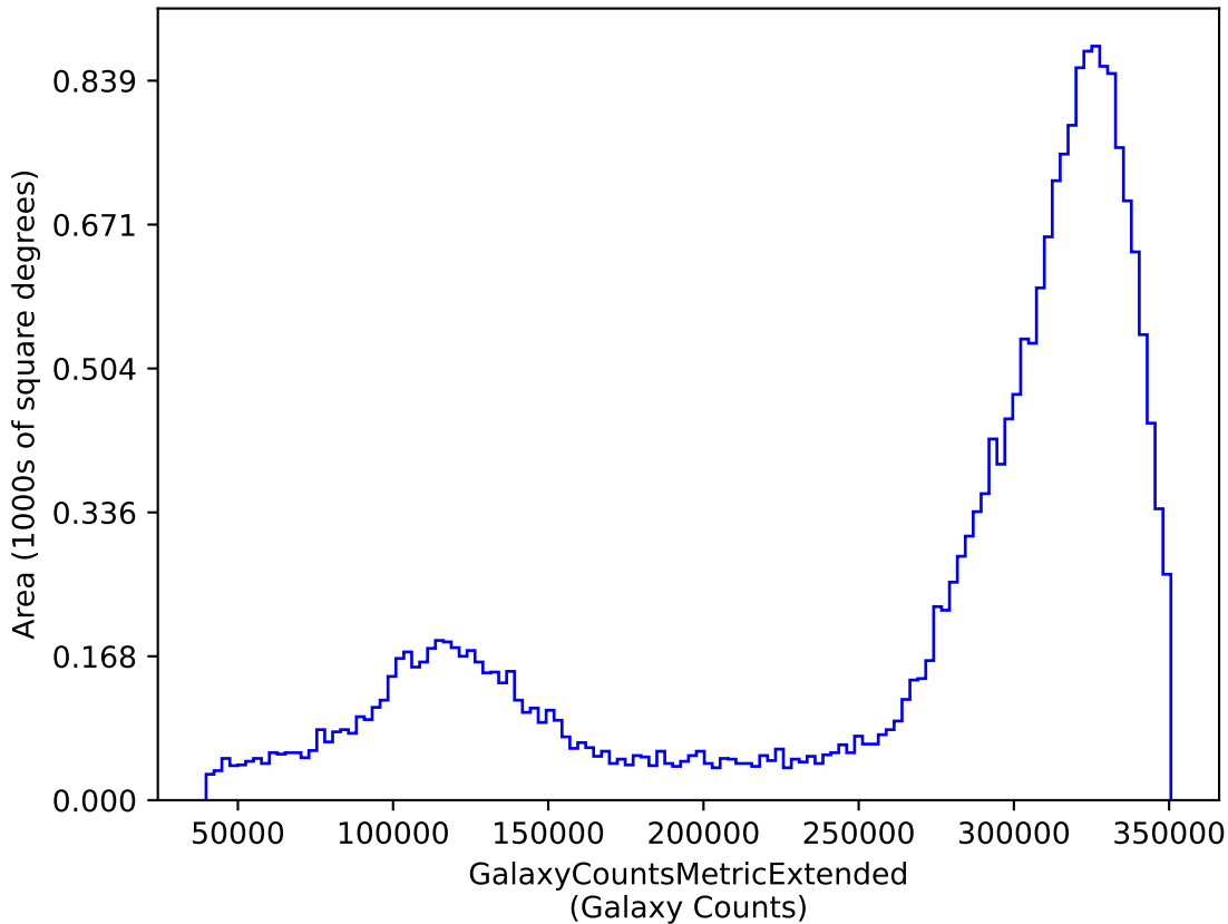
weather_cloudso8v3.5_10yrs y: GalaxyCountsMetricExtended
