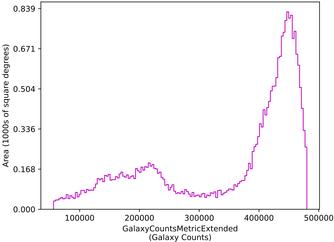
weather_cloudso8v3.5_10yrs z: GalaxyCountsMetricExtended
